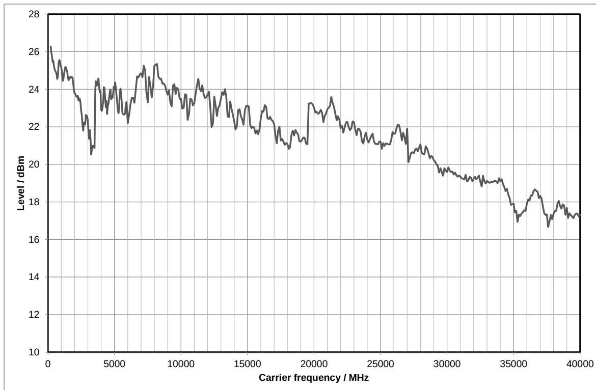
Measured maximum available output level versus frequency with R&S®SMW-B1040, R&S®SMW-B1040N frequency options
